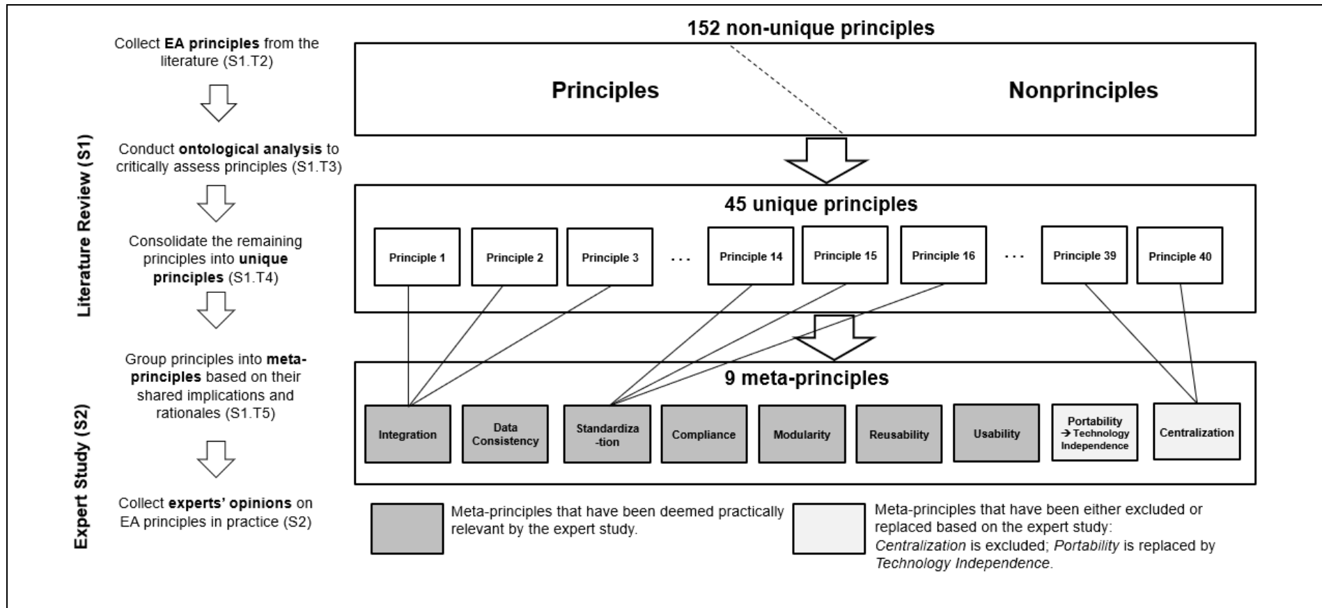
Figure 1: The Investigation of Suitable EA Principles (RQ1)
