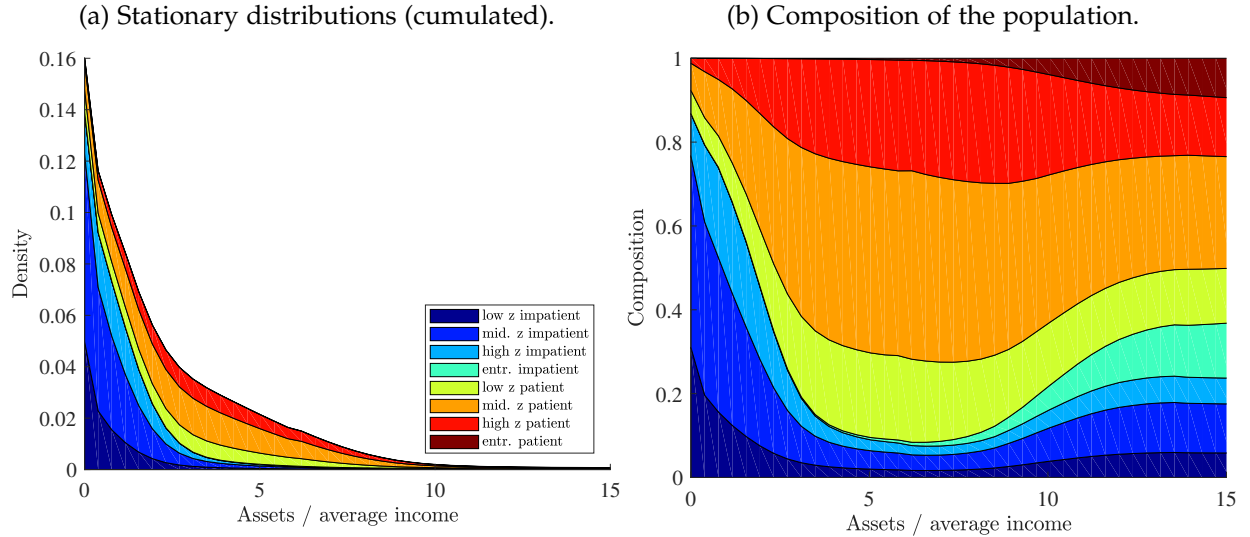
Figure 1: Stationary distributions
